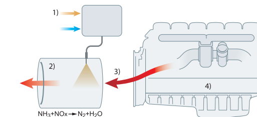
1) Urea, 2) Catalytic converter, 3) Exhaust gas, 4) Engine
